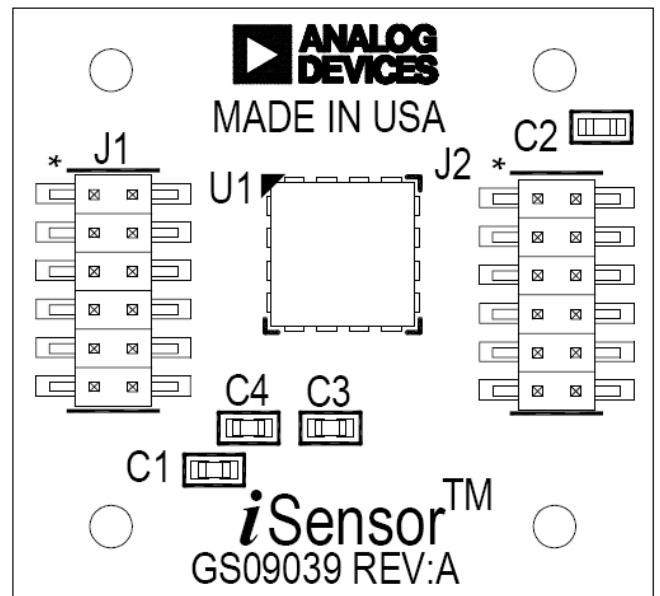
Figure 2 - ADIS16080/PCB Layout (Top View)
